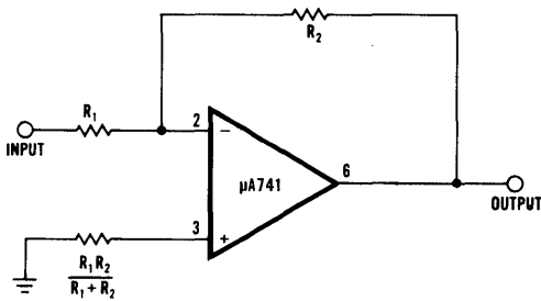
INVERTING AMPLIFIER
